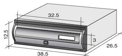
CURVE 1 completa - CURVE 1 complete box
