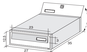
MODULAR 270/2 completa MODULAR 270/2 complete box
