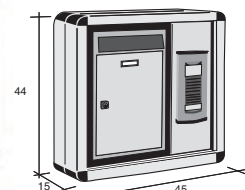
Combi 3/2 - cornice - external frame PRELIEVO POSTERIORE - REAR ACCESS
